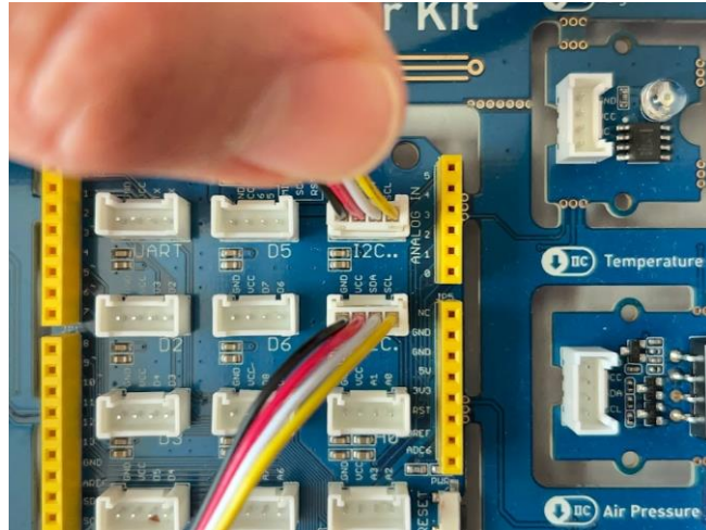
Grove CO2 and VOC/NOx sensor plugged into the Grove Beginner Kit For Arduino.
