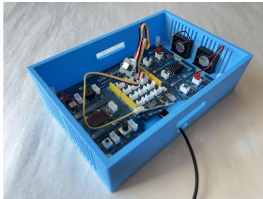
Internals of assembled RADBox.
