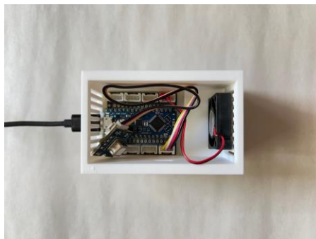
Internals of assembled RADBox Lite.
